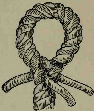
FIG. 108.—Eye splice.
